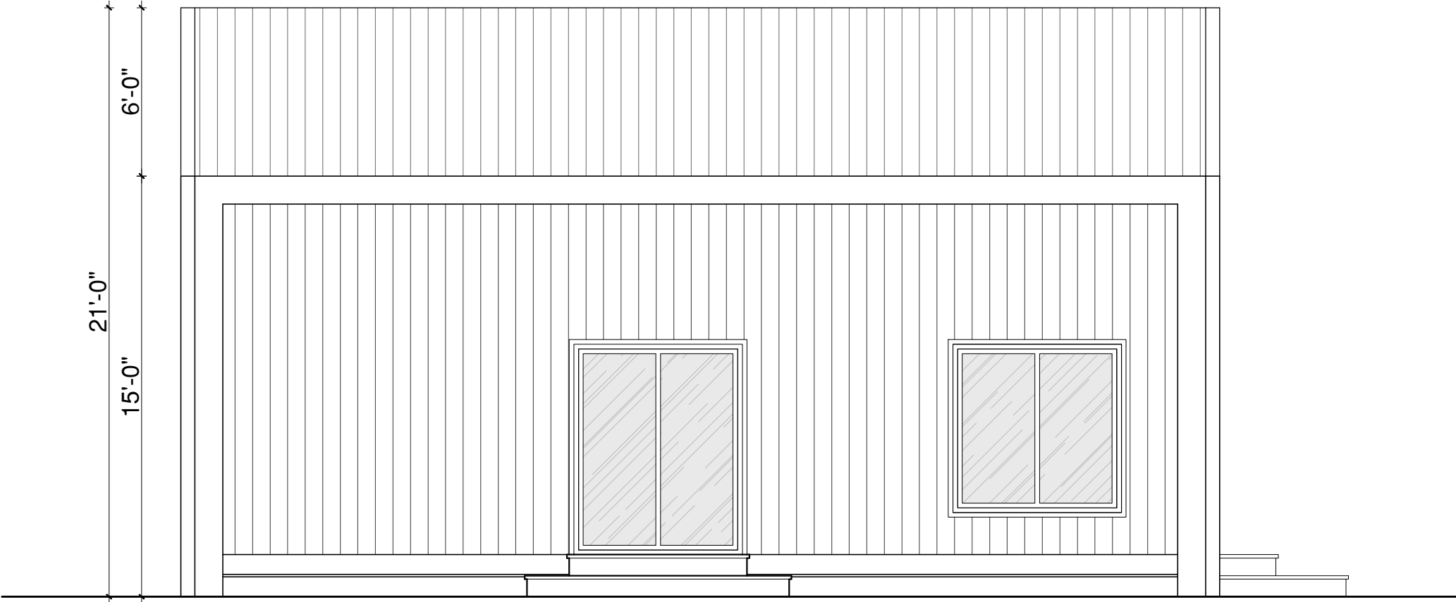
LEFT ELEVATION
